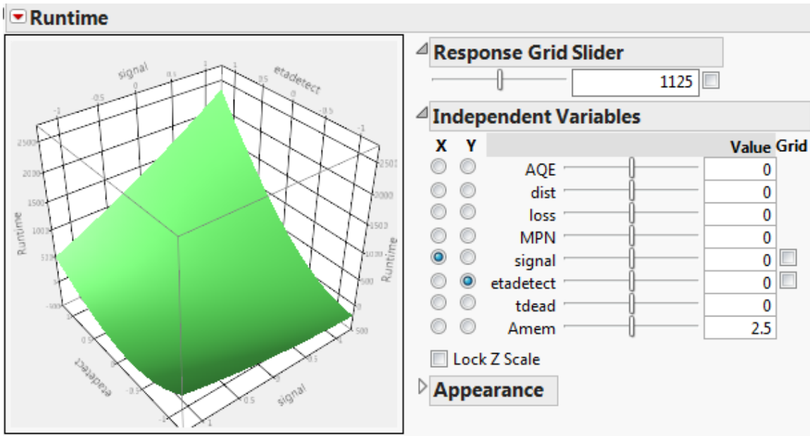
Figure 44. Surface profile of signal vs. etadetect
